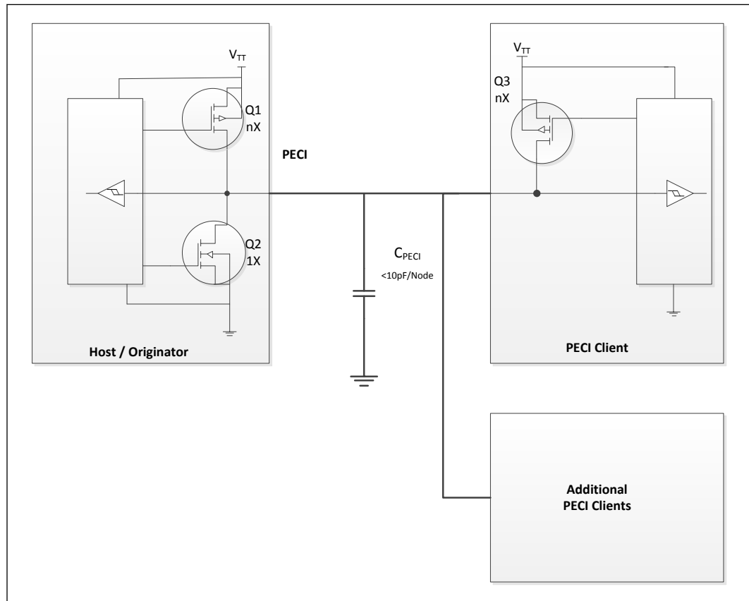
Figure 9. Example for PECI Host-Clients Connection
