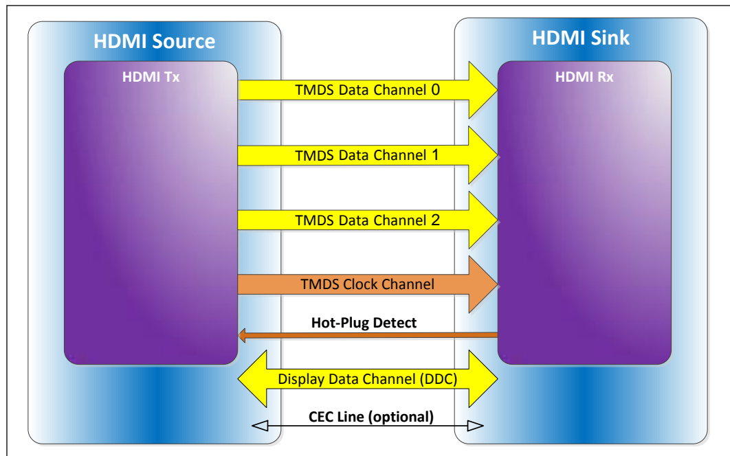
Figure 8. HDMI* Overview
