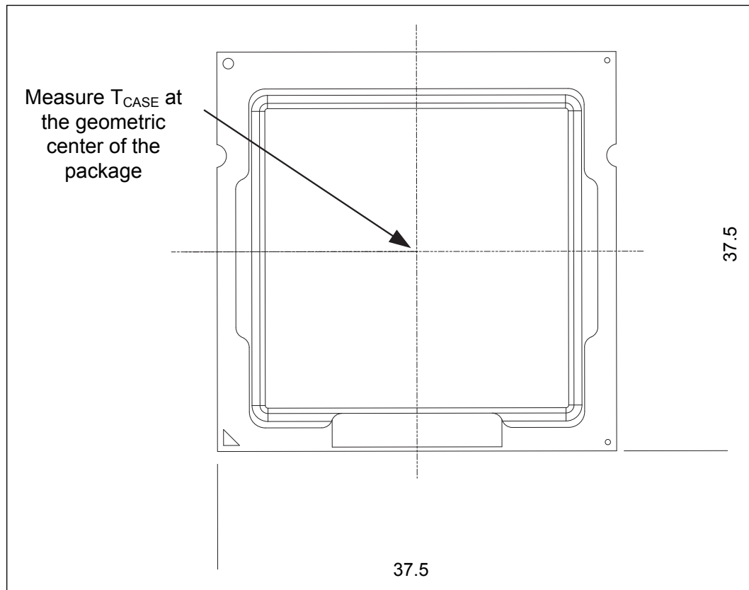
Figure 15. Thermal Test Vehicle (TTV) Case Temperature ( T_{CASE} ) Measurement Location
