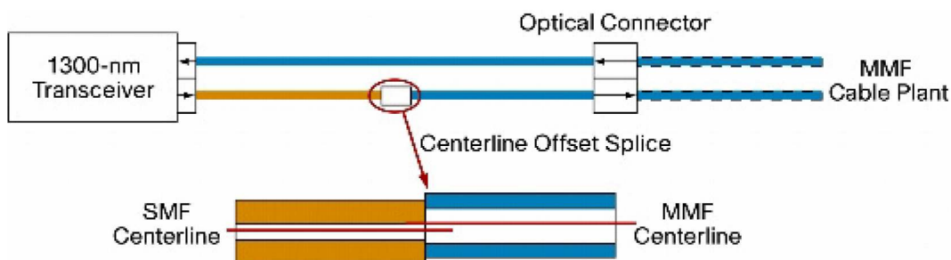
Figure 1. Mode Conditioning Patch Cable Installation
