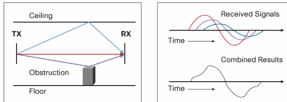
Figure 4. Multipath Distortion
